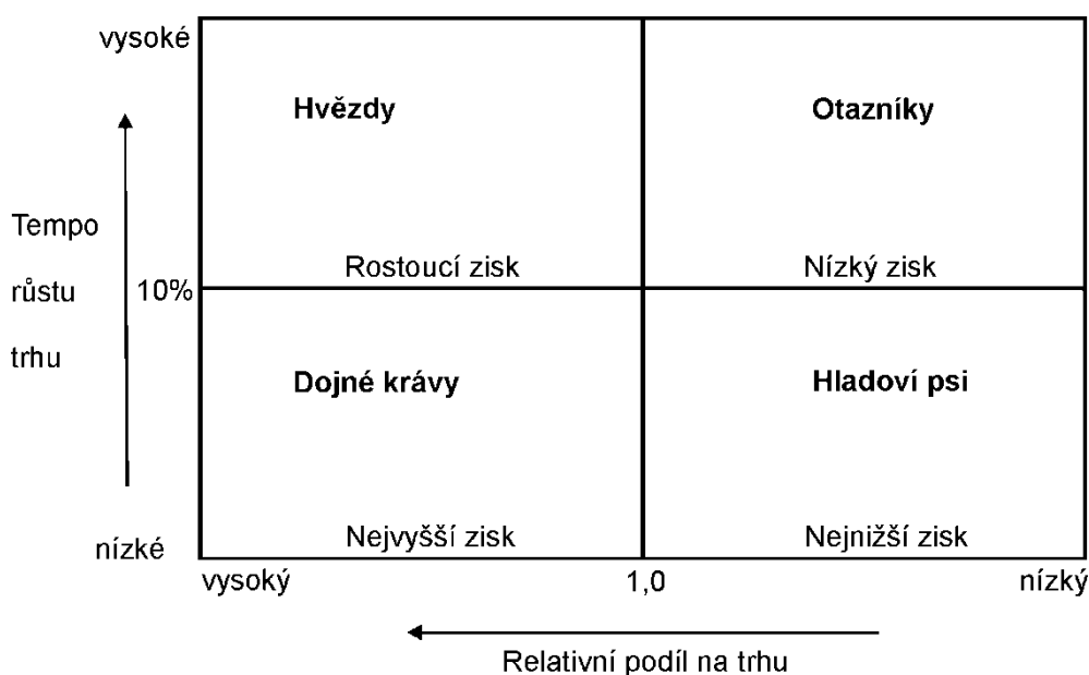
Obr. 11 BCG model [20]
